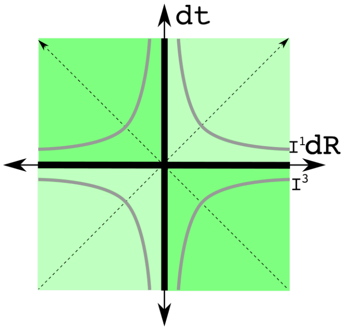
Gravity
