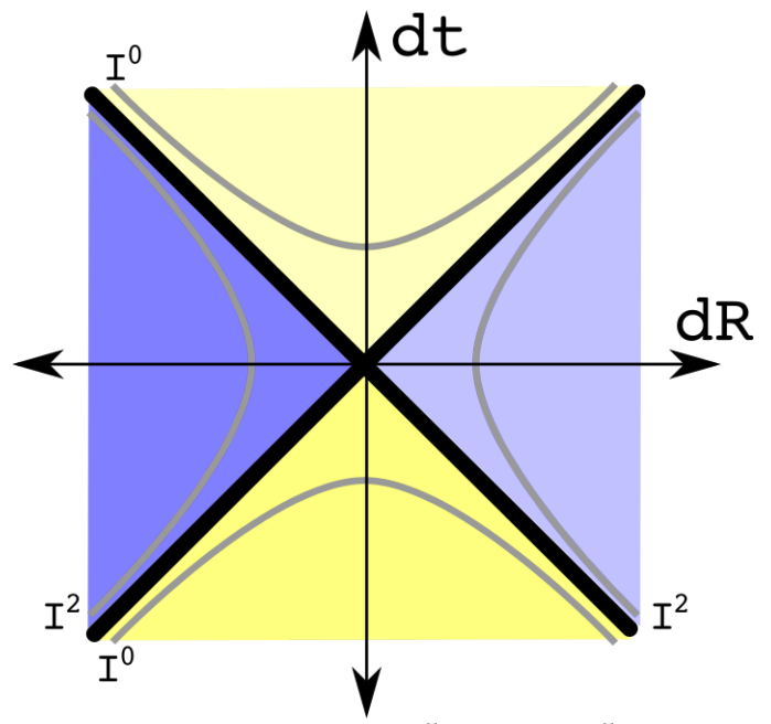
Special Rel
