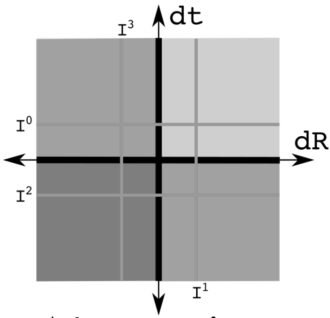
Newtonian
